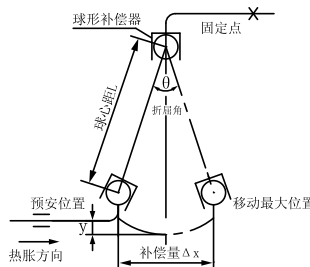
图1 球形补偿器工作原理图 FIG. 1 working principle diagram of spherical compensator
