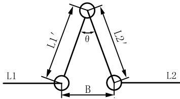
图5 \Omega 型组合补偿器正面图 Figure 5 Positive figure of \Omega type combined compensator
