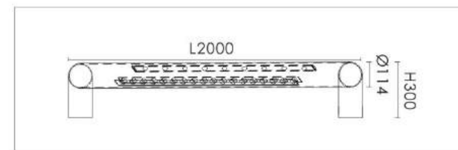
线条尺寸图/Line size chart
