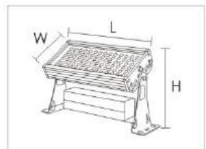
线条尺寸图/Line size chart
