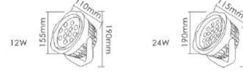
线条尺寸图/Line size chart
