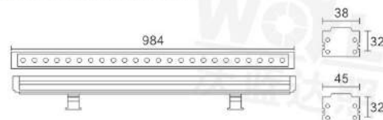
线条尺寸图/Line size chart
