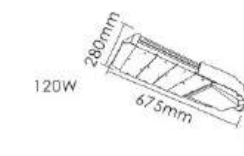
线条尺寸图/Line size chart
