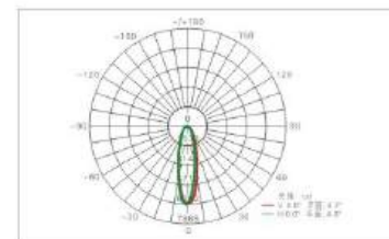
配光曲线图/Light distribution curve
