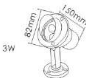
线条尺寸图/Line size chart
