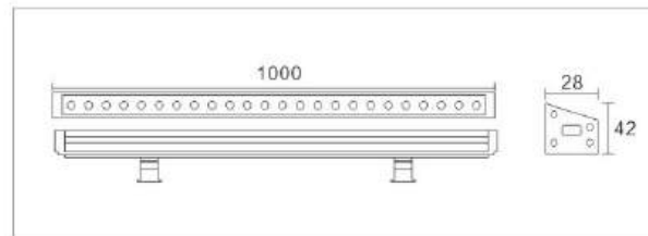
线条尺寸图/Line size chart
