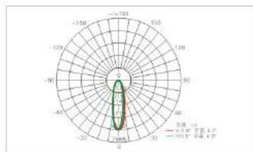
配光曲线图/Light distribution curve
