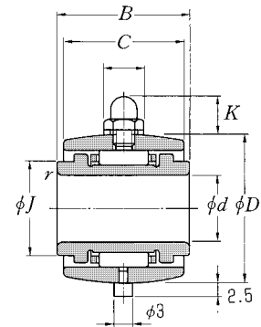
Type FRIS · · NP (With grease nipple/knock pin) 2)
