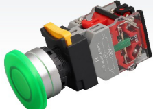
HBS0-KW-□MD/△/201 Ø22mm Illuminated Mushroom Head Pushbuttons 带灯蘑菇头按钮
